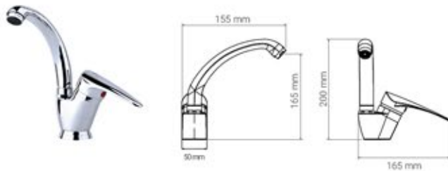
Basin Mixer
