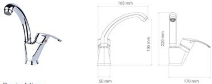
Basin Mixer
