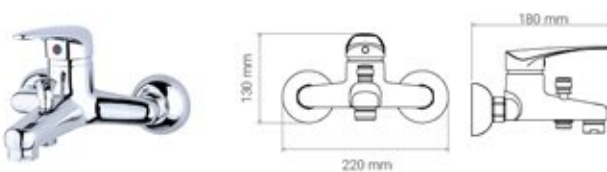
Bath Mixer
