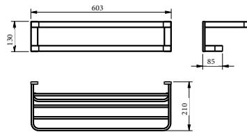
BL112 CV78 Double towel rack Material:SUS304
