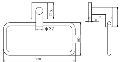
BL004 TZ C Towel ring Material:SUS304
