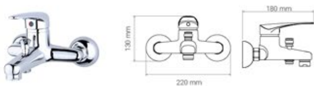
Bath Mixer
