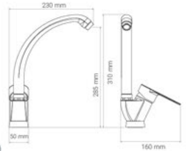
Basin Mixer (swivel spout)
