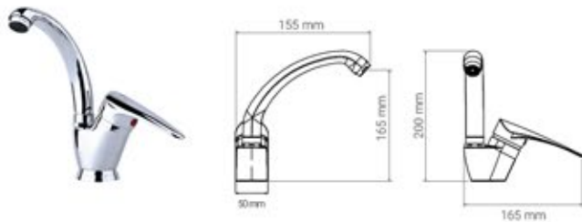
Basin Mixer
