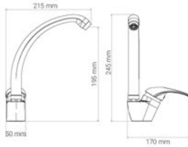
Basin Mixer (swivel spout)
