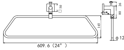
BL104 TZ C Towel ring Material:SUS304
